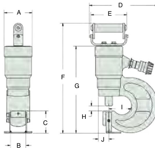
Punch Dimensions
